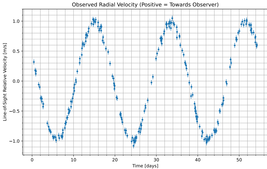
Figure 1: We have isolated the radial velocity of the host star due to the candidate planet. Data begins at UTC 2088-09-25/15:26. Positive values indicate the velocity at which the star is moving towards us; negative indicate the velocity at which it is moving away.
