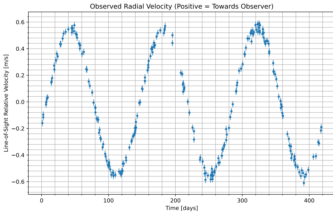
Figure 1: We have isolated the radial velocity of the host star due to the candidate planet. Data begins at UTC 2083-04-12/10:16. Positive values indicate the velocity at which the star is moving towards us; negative indicate the velocity at which it is moving away.
