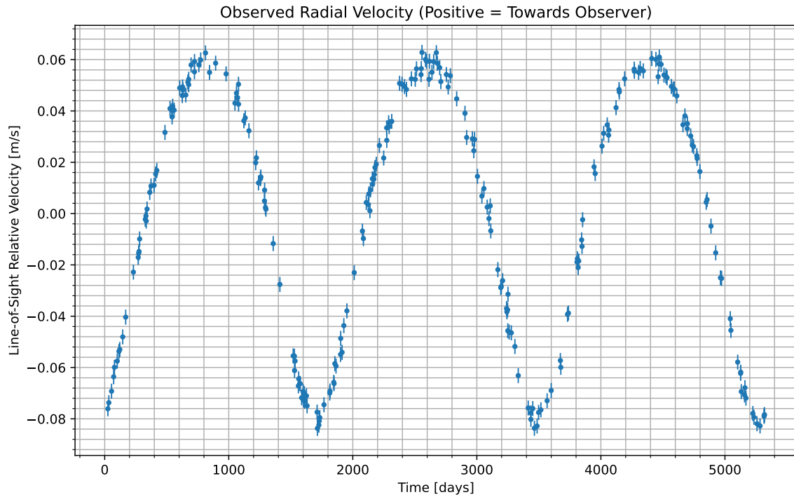
Figure 1: We have isolated the radial velocity of the host star due to the candidate planet. Data begins at UTC 2074-04-04/16:48. Positive values indicate the velocity at which the star is moving towards us; negative indicate the velocity at which it is moving away.
