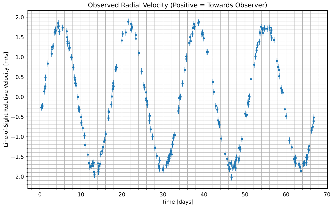
Figure 1: We have isolated the radial velocity of the host star due to the candidate planet. Data begins at UTC 2077-12-23/00:28. Positive values indicate the velocity at which the star is moving towards us; negative indicate the velocity at which it is moving away.
