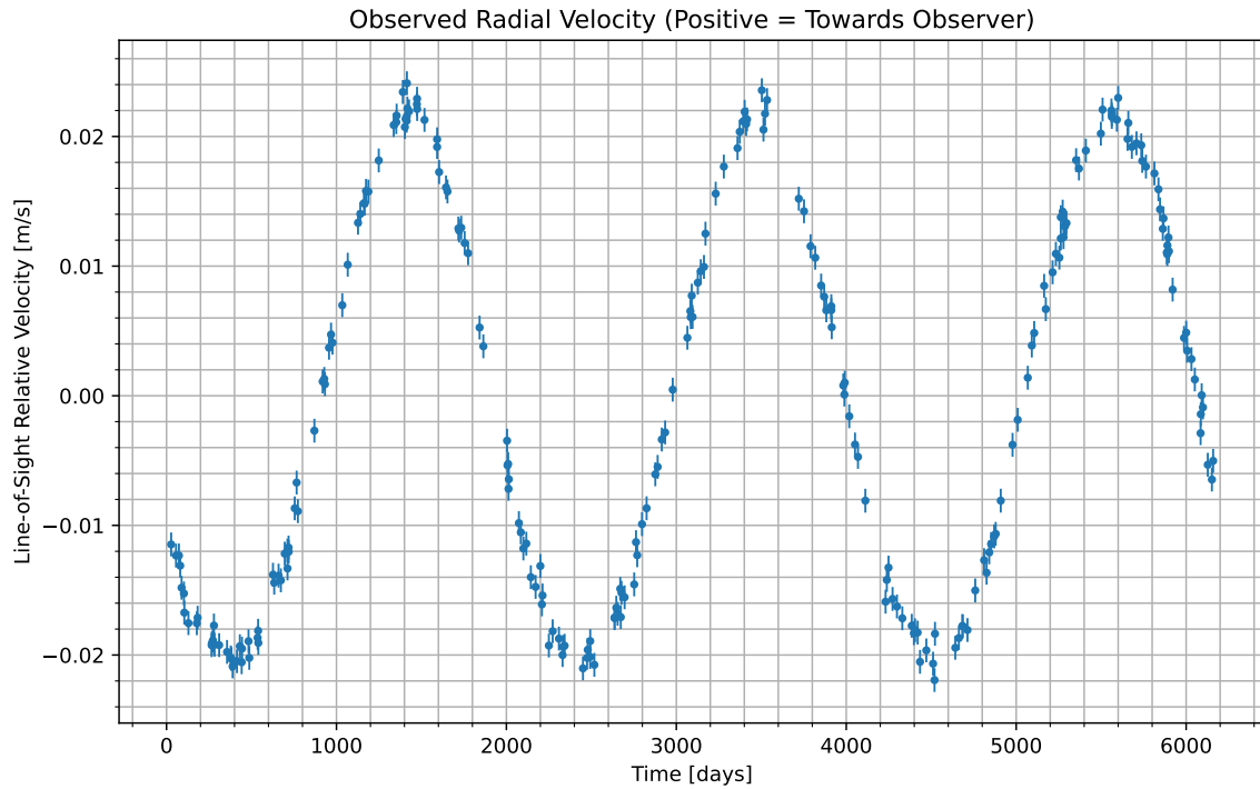
Figure 1: We have isolated the radial velocity of the host star due to the candidate planet. Data begins at UTC 2066-07-07/00:11. Positive values indicate the velocity at which the star is moving towards us; negative indicate the velocity at which it is moving away.
