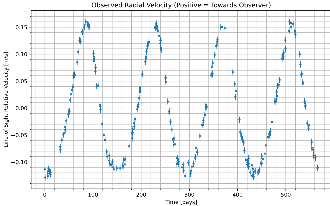
Figure 1: We have isolated the radial velocity of the host star due to the candidate planet. Data begins at UTC 2092-09-21/15:11. Positive values indicate the velocity at which the star is moving towards us; negative indicate the velocity at which it is moving away.
