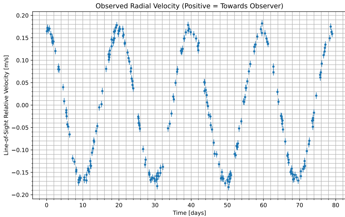
Figure 1: We have isolated the radial velocity of the host star due to the candidate planet. Data begins at UTC 2094-08-21/07:49. Positive values indicate the velocity at which the star is moving towards us; negative indicate the velocity at which it is moving away.
