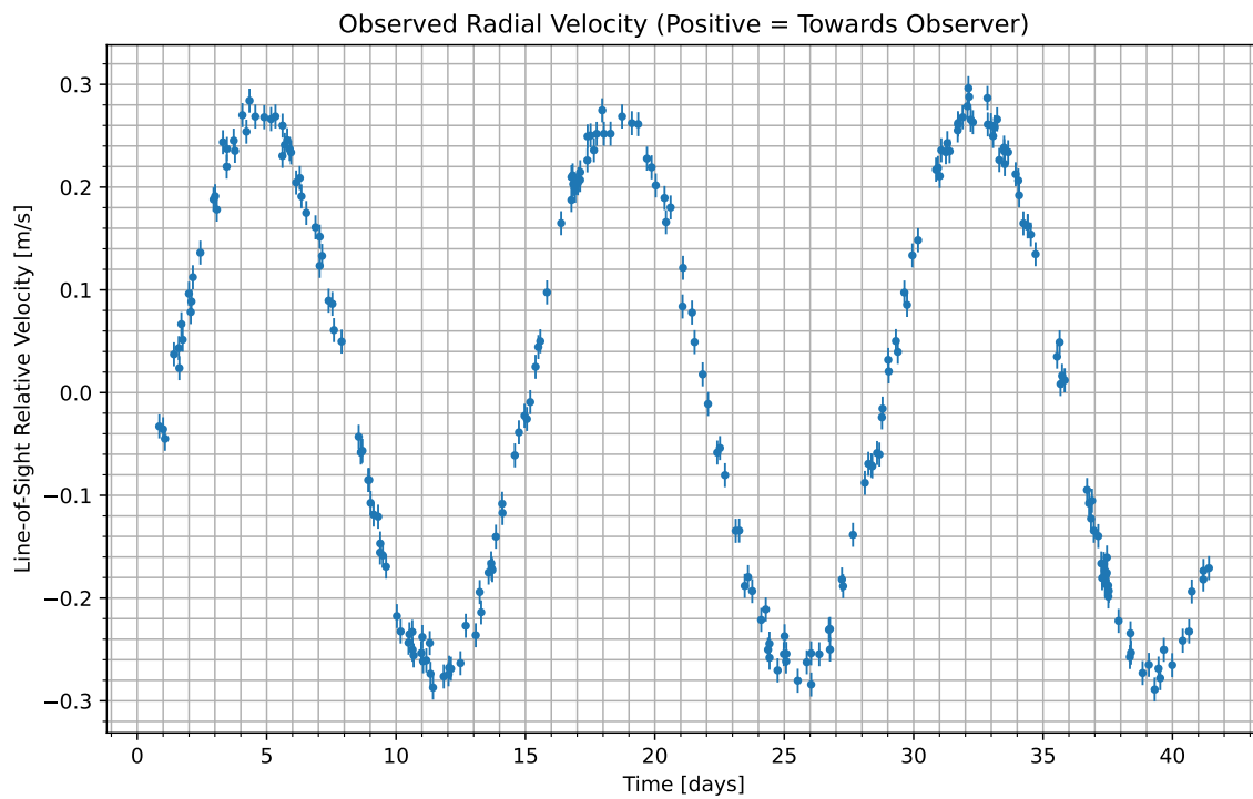
Figure 1: We have isolated the radial velocity of the host star due to the candidate planet. Data begins at UTC 2080-02-20/19:21. Positive values indicate the velocity at which the star is moving towards us; negative indicate the velocity at which it is moving away.
