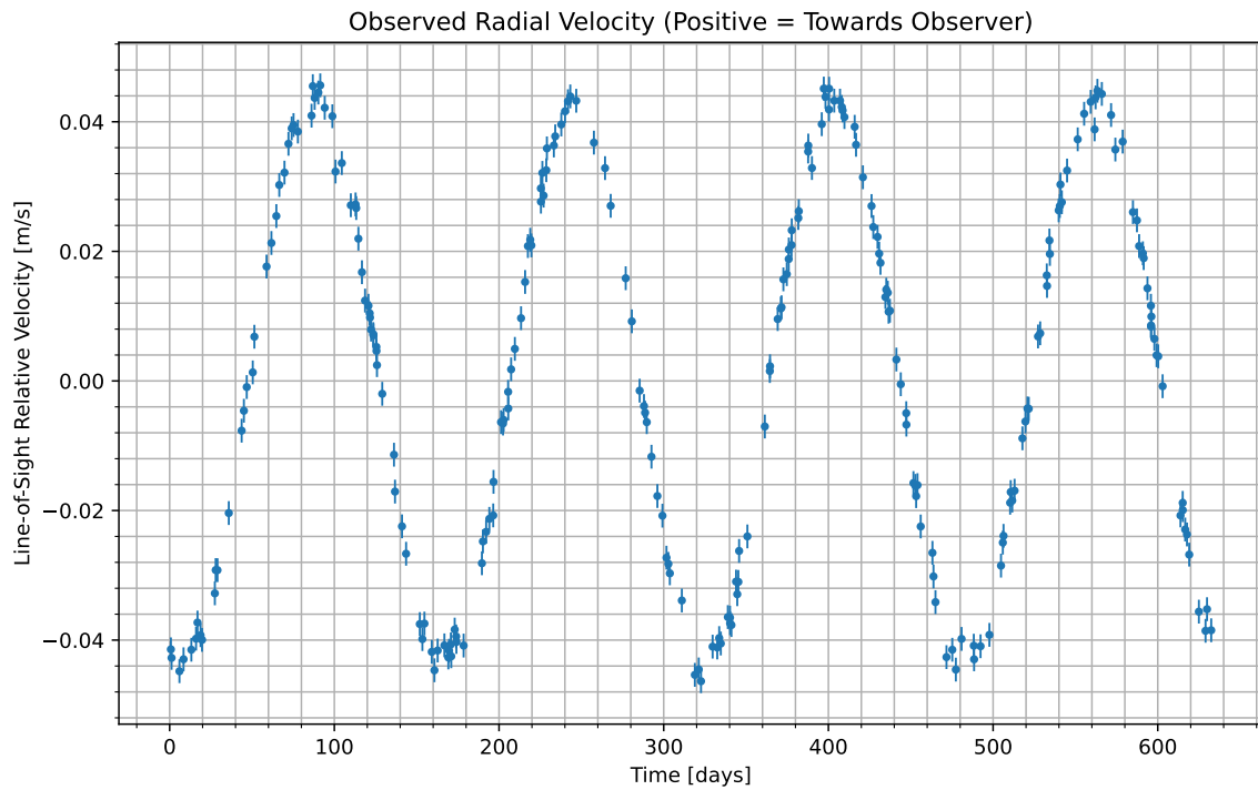
Figure 1: We have isolated the radial velocity of the host star due to the candidate planet. Data begins at UTC 2088-08-05/21:40. Positive values indicate the velocity at which the star is moving towards us; negative indicate the velocity at which it is moving away.
