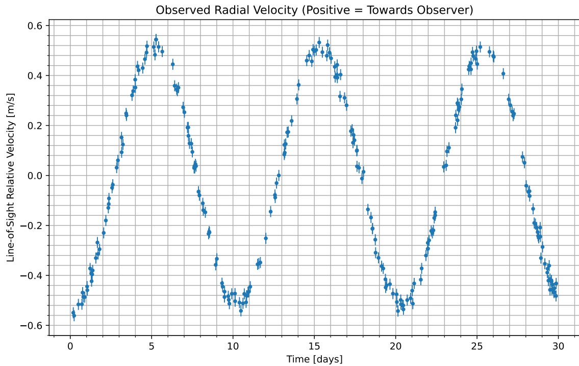
Figure 1: We have isolated the radial velocity of the host star due to the candidate planet. Data begins at UTC 2090-07-26/19:36. Positive values indicate the velocity at which the star is moving towards us; negative indicate the velocity at which it is moving away.
