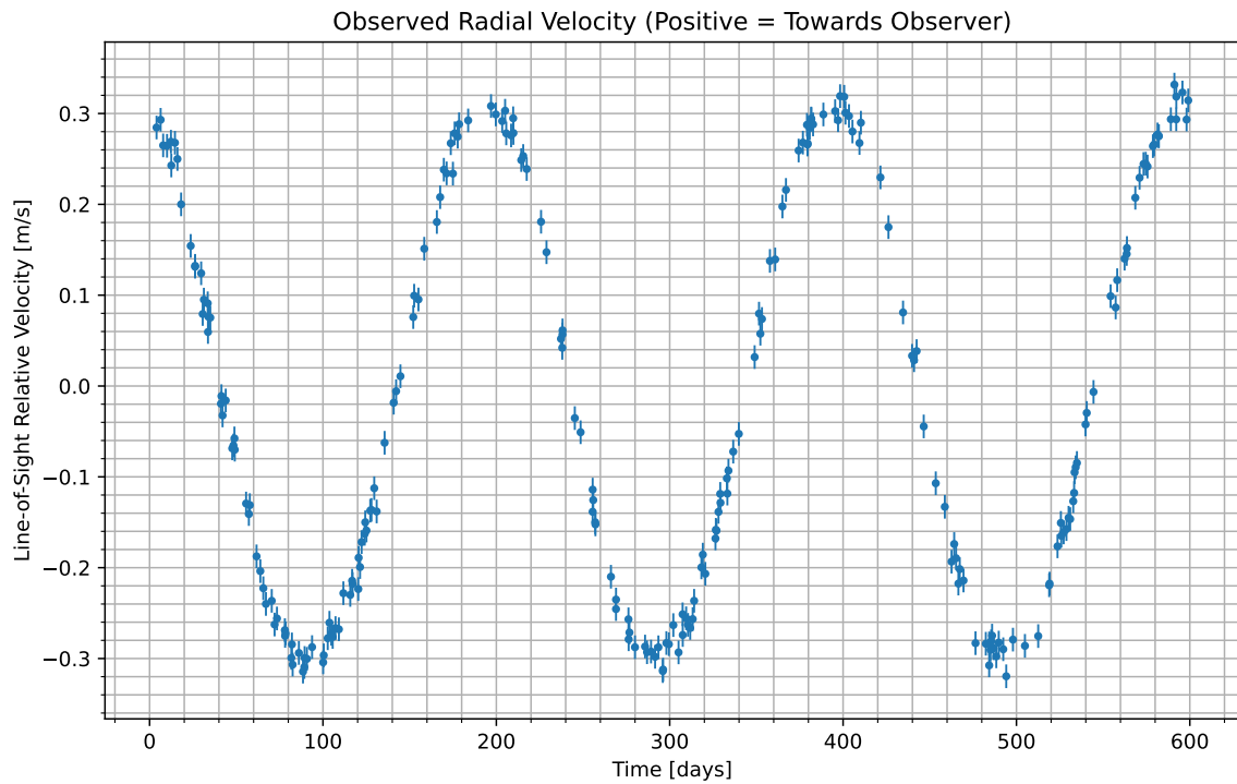
Figure 1: We have isolated the radial velocity of the host star due to the candidate planet. Data begins at UTC 2084-05-07/14:40. Positive values indicate the velocity at which the star is moving towards us; negative indicate the velocity at which it is moving away.
