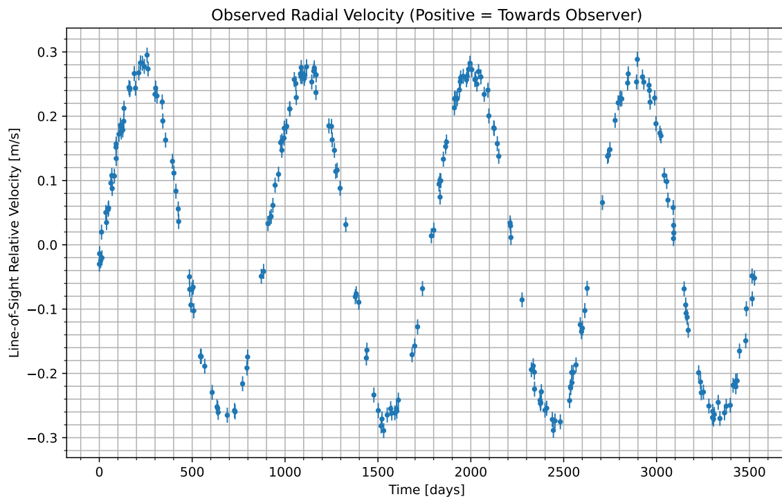
Figure 1: We have isolated the radial velocity of the host star due to the candidate planet. Data begins at UTC 2073-12-17/08:19. Positive values indicate the velocity at which the star is moving towards us; negative indicate the velocity at which it is moving away.
