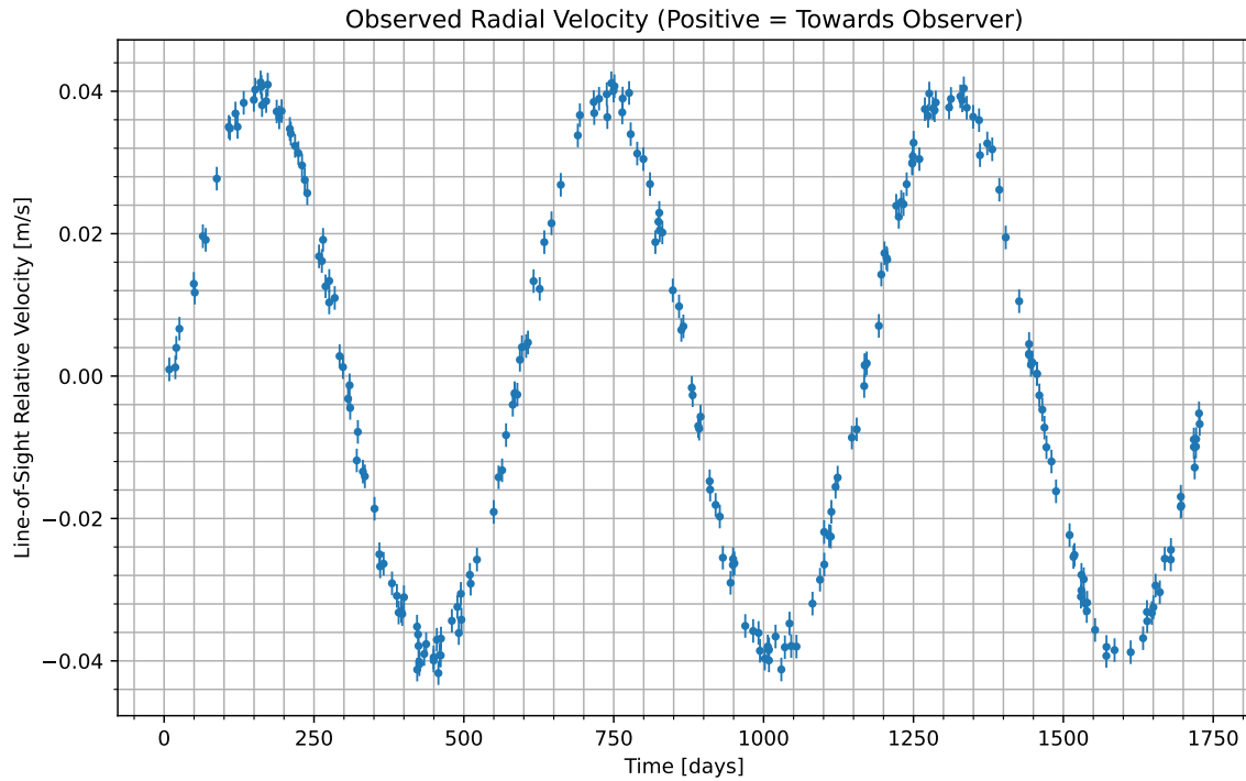
Figure 1: We have isolated the radial velocity of the host star due to the candidate planet. Data begins at UTC 2081-10-16/16:52. Positive values indicate the velocity at which the star is moving towards us; negative indicate the velocity at which it is moving away.
