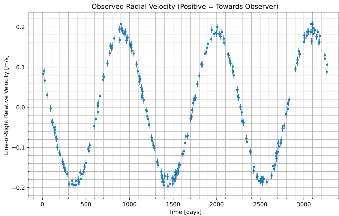
Figure 1: We have isolated the radial velocity of the host star due to the candidate planet. Data begins at UTC 2083-07-01/13:23. Positive values indicate the velocity at which the star is moving towards us; negative indicate the velocity at which it is moving away.
