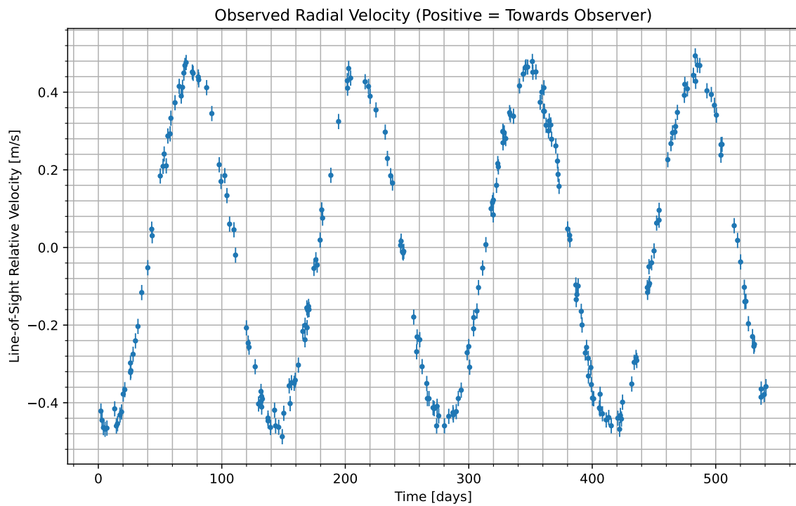
Figure 1: We have isolated the radial velocity of the host star due to the candidate planet. Data begins at UTC 2090-07-10/10:26. Positive values indicate the velocity at which the star is moving towards us; negative indicate the velocity at which it is moving away.
