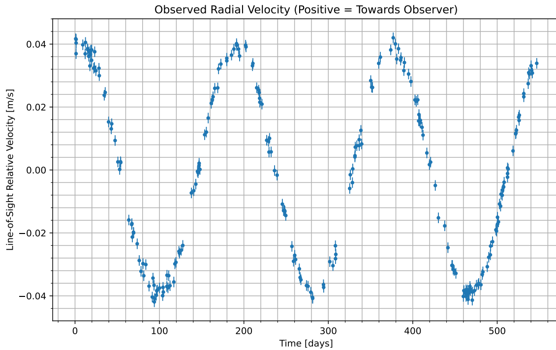
Figure 1: We have isolated the radial velocity of the host star due to the candidate planet. Data begins at UTC 2086-05-09/23:30. Positive values indicate the velocity at which the star is moving towards us; negative indicate the velocity at which it is moving away.
