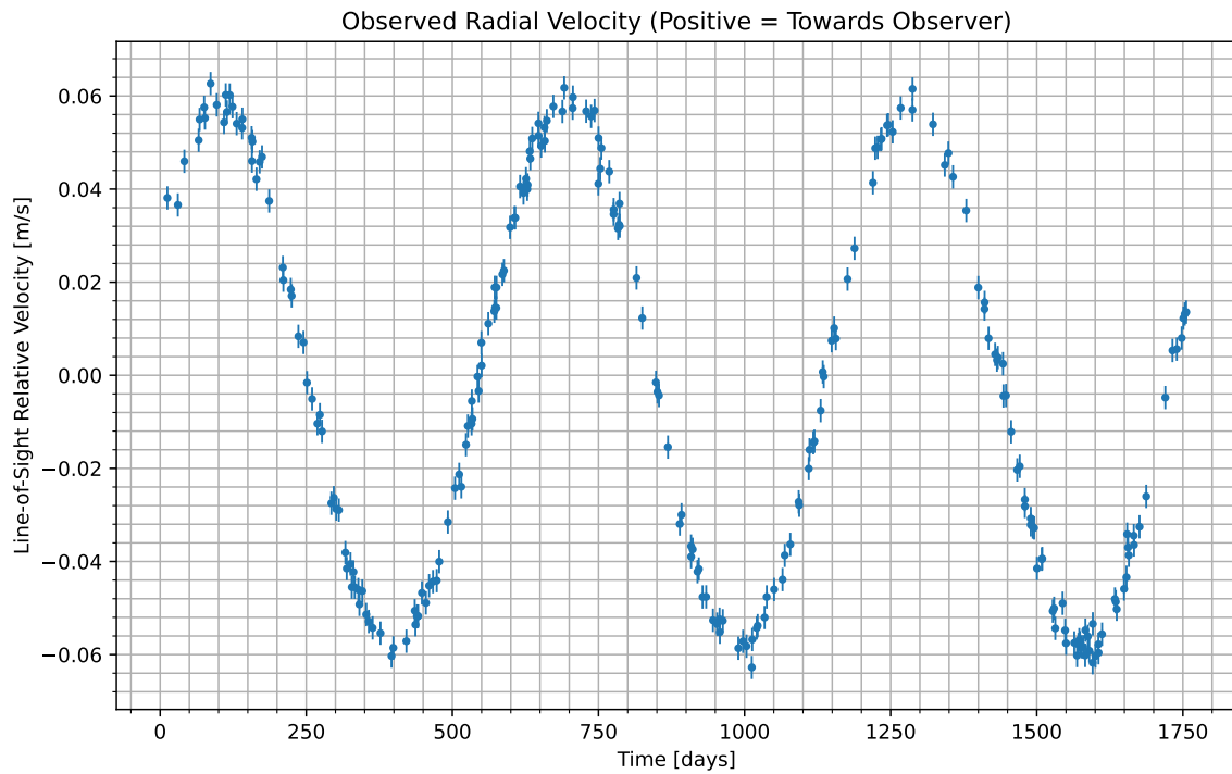
Figure 1: We have isolated the radial velocity of the host star due to the candidate planet. Data begins at UTC 2077-12-03/04:17. Positive values indicate the velocity at which the star is moving towards us; negative indicate the velocity at which it is moving away.
