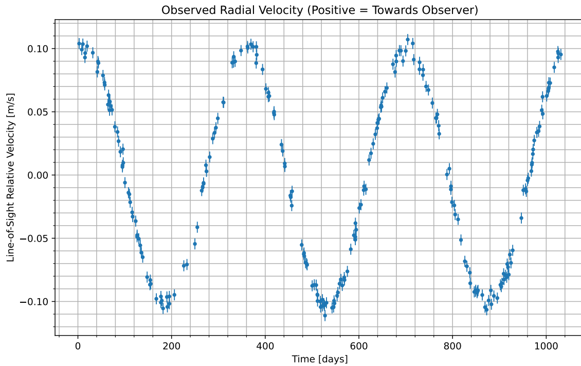
Figure 1: We have isolated the radial velocity of the host star due to the candidate planet. Data begins at UTC 2079-10-09/00:15. Positive values indicate the velocity at which the star is moving towards us; negative indicate the velocity at which it is moving away.
