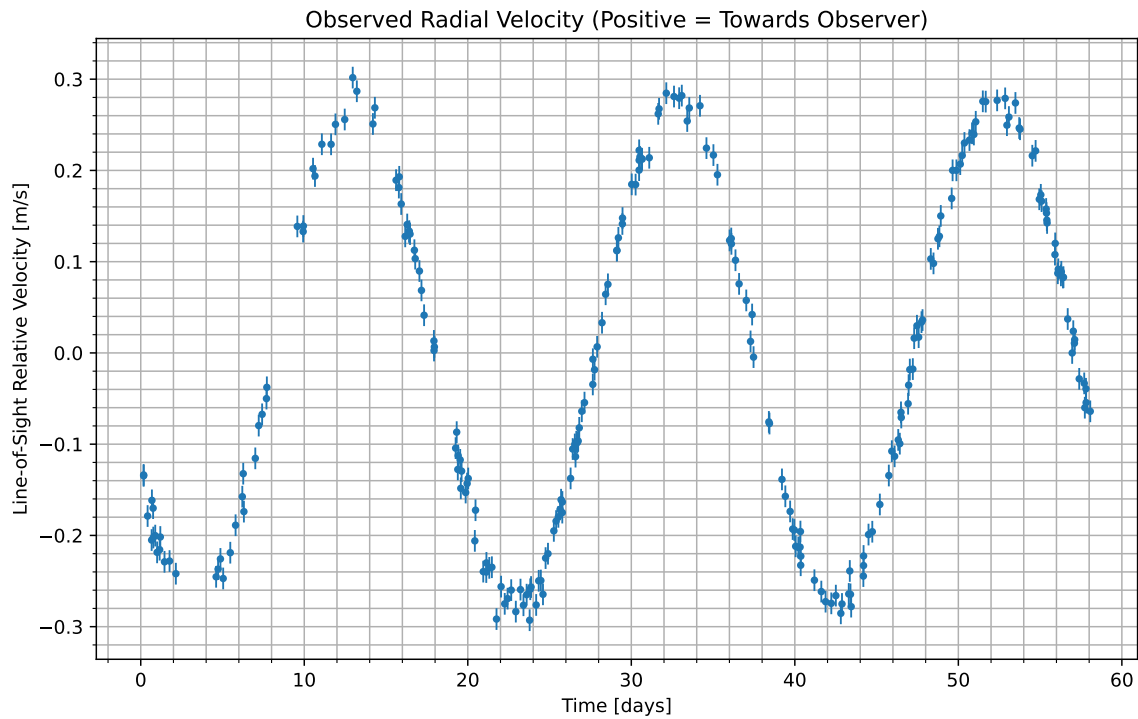
Figure 1: We have isolated the radial velocity of the host star due to the candidate planet. Data begins at UTC 2074-04-13/12:38. Positive values indicate the velocity at which the star is moving towards us; negative indicate the velocity at which it is moving away.
