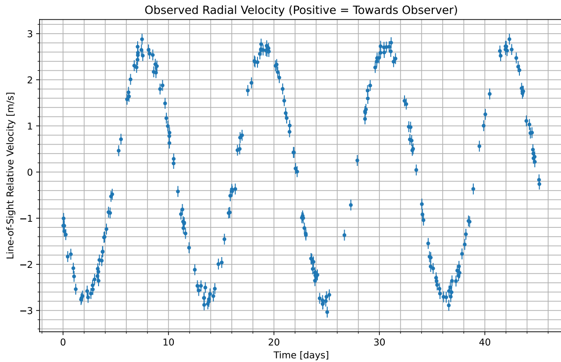
Figure 1: We have isolated the radial velocity of the host star due to the candidate planet. Data begins at UTC 2076-08-30/01:37. Positive values indicate the velocity at which the star is moving towards us; negative indicate the velocity at which it is moving away.
