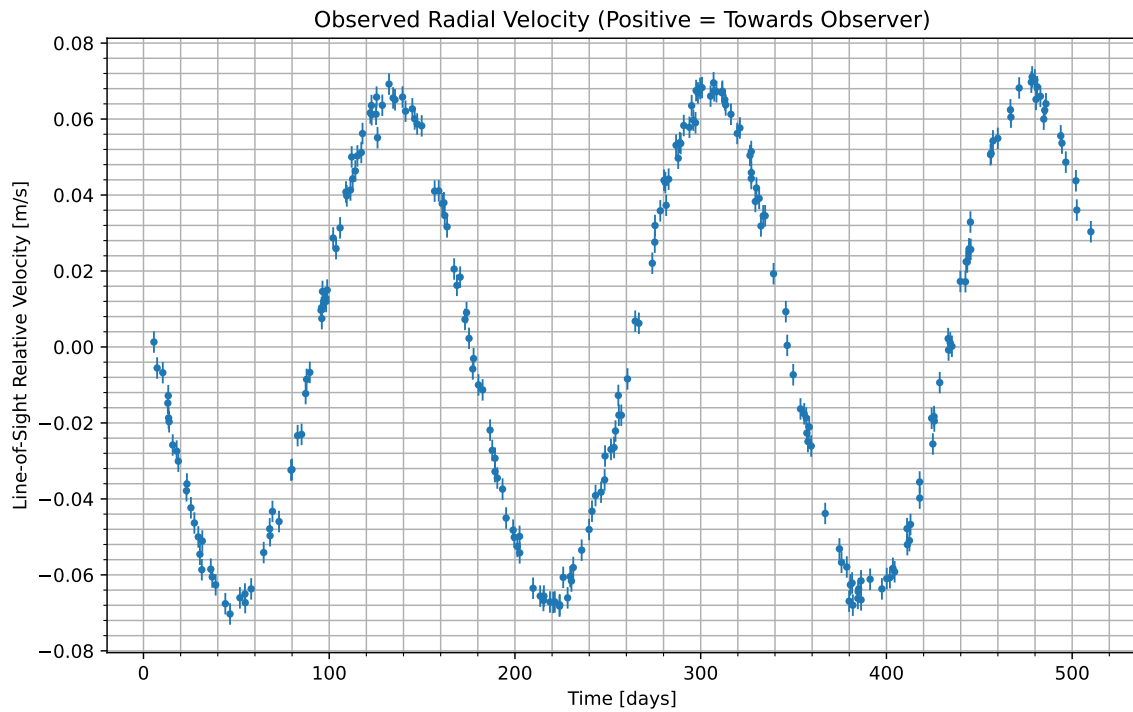
Figure 1: We have isolated the radial velocity of the host star due to the candidate planet. Data begins at UTC 2093-04-15/14:13. Positive values indicate the velocity at which the star is moving towards us; negative indicate the velocity at which it is moving away.
