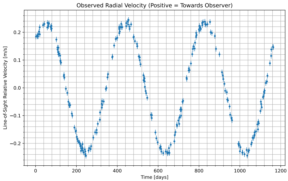
Figure 1: We have isolated the radial velocity of the host star due to the candidate planet. Data begins at UTC 2096-05-07/19:33. Positive values indicate the velocity at which the star is moving towards us; negative indicate the velocity at which it is moving away.
