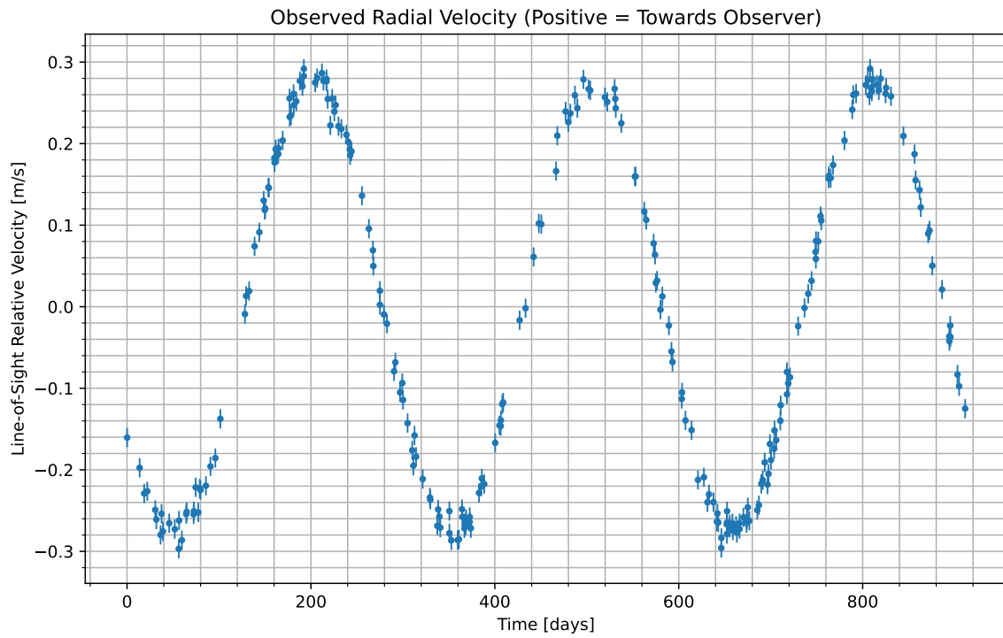
Figure 1: We have isolated the radial velocity of the host star due to the candidate planet. Data begins at UTC 2094-07-24/00:05. Positive values indicate the velocity at which the star is moving towards us; negative indicate the velocity at which it is moving away.
