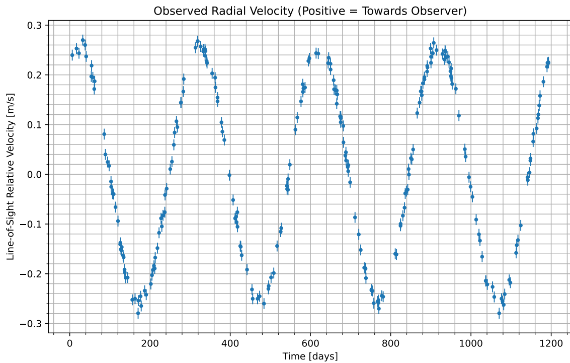
Figure 1: We have isolated the radial velocity of the host star due to the candidate planet. Data begins at UTC 2086-01-03/10:51. Positive values indicate the velocity at which the star is moving towards us; negative indicate the velocity at which it is moving away.
