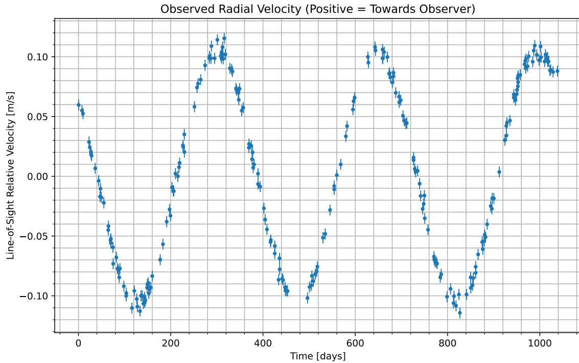
Figure 1: We have isolated the radial velocity of the host star due to the candidate planet. Data begins at UTC 2082-05-31/07:13. Positive values indicate the velocity at which the star is moving towards us; negative indicate the velocity at which it is moving away.
