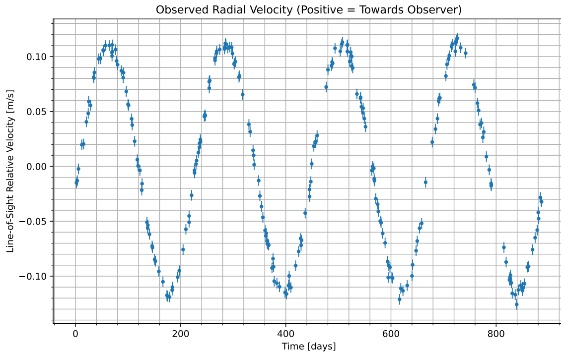
Figure 1: We have isolated the radial velocity of the host star due to the candidate planet. Data begins at UTC 2068-07-15/01:11. Positive values indicate the velocity at which the star is moving towards us; negative indicate the velocity at which it is moving away.
