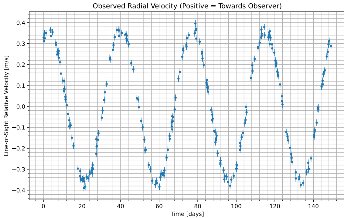
Figure 1: We have isolated the radial velocity of the host star due to the candidate planet. Data begins at UTC 2077-01-08/23:49. Positive values indicate the velocity at which the star is moving towards us; negative indicate the velocity at which it is moving away.
