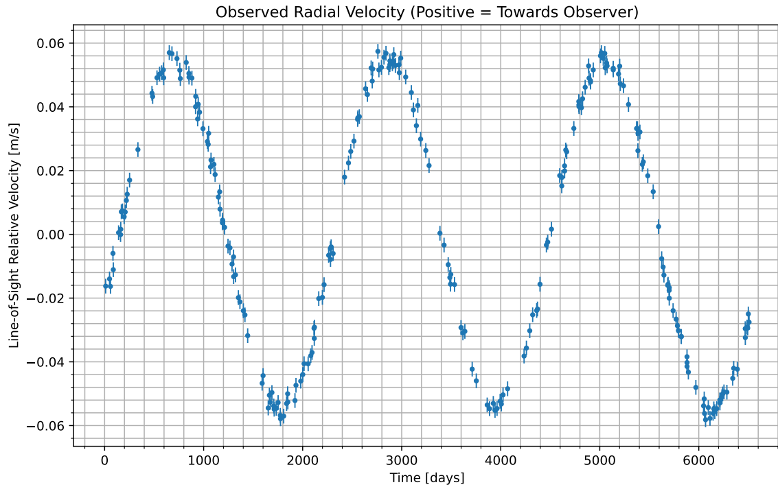
Figure 1: We have isolated the radial velocity of the host star due to the candidate planet. Data begins at UTC 2070-04-18/03:28. Positive values indicate the velocity at which the star is moving towards us; negative indicate the velocity at which it is moving away.
