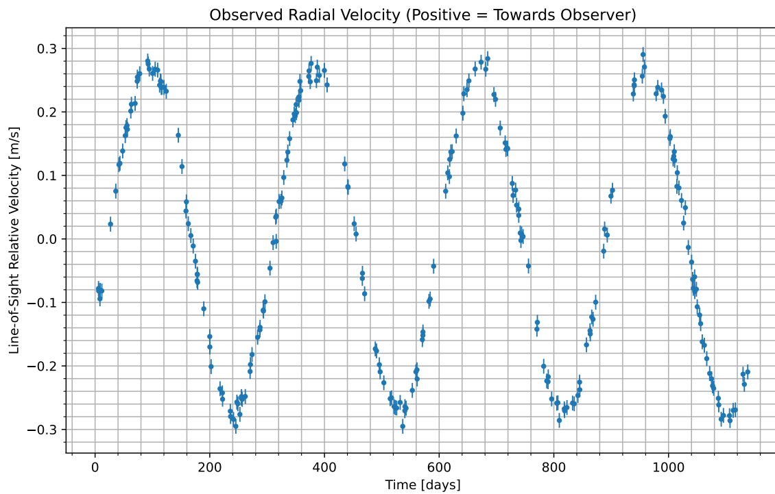
Figure 1: We have isolated the radial velocity of the host star due to the candidate planet. Data begins at UTC 2083-07-24/06:34. Positive values indicate the velocity at which the star is moving towards us; negative indicate the velocity at which it is moving away.
