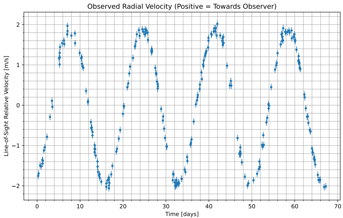
Figure 1: We have isolated the radial velocity of the host star due to the candidate planet. Data begins at UTC 2094-08-27/21:06. Positive values indicate the velocity at which the star is moving towards us; negative indicate the velocity at which it is moving away.
