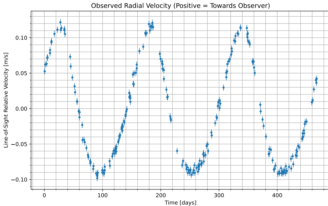
Figure 1: We have isolated the radial velocity of the host star due to the candidate planet. Data begins at UTC 2091-06-19/11:23. Positive values indicate the velocity at which the star is moving towards us; negative indicate the velocity at which it is moving away.
