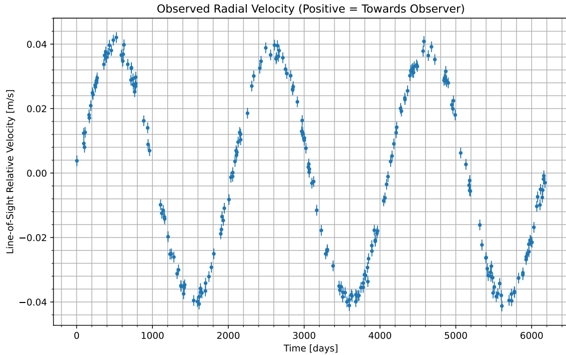
Figure 1: We have isolated the radial velocity of the host star due to the candidate planet. Data begins at UTC 2061-02-09/08:42. Positive values indicate the velocity at which the star is moving towards us; negative indicate the velocity at which it is moving away.
