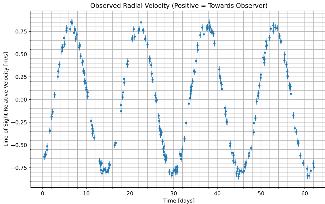
Figure 1: We have isolated the radial velocity of the host star due to the candidate planet. Data begins at UTC 2089-05-14/03:50. Positive values indicate the velocity at which the star is moving towards us; negative indicate the velocity at which it is moving away.
