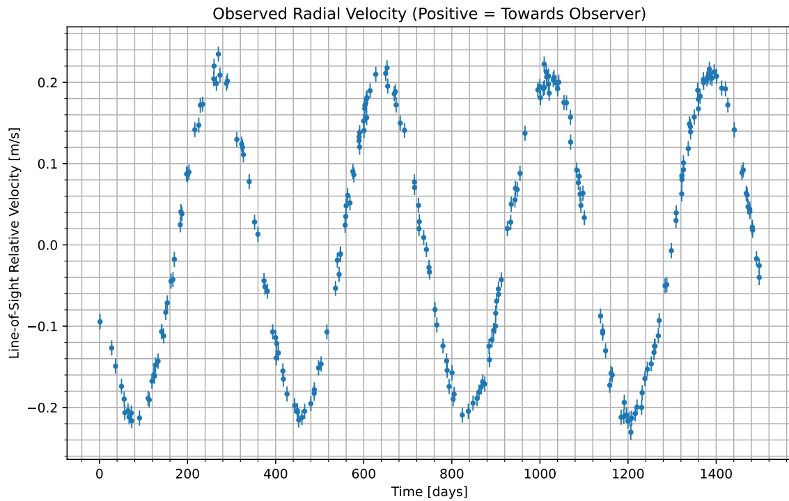
Figure 1: We have isolated the radial velocity of the host star due to the candidate planet. Data begins at UTC 2093-12-31/05:22. Positive values indicate the velocity at which the star is moving towards us; negative indicate the velocity at which it is moving away.
