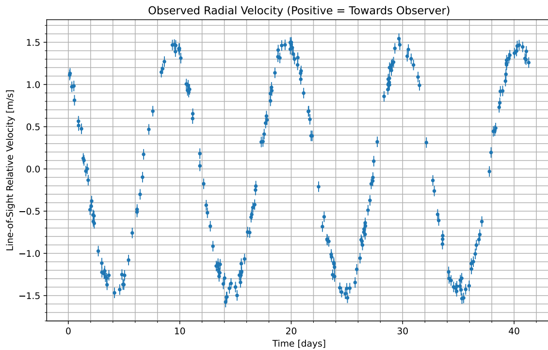
Figure 1: We have isolated the radial velocity of the host star due to the candidate planet. Data begins at UTC 2077-04-16/13:51. Positive values indicate the velocity at which the star is moving towards us; negative indicate the velocity at which it is moving away.
