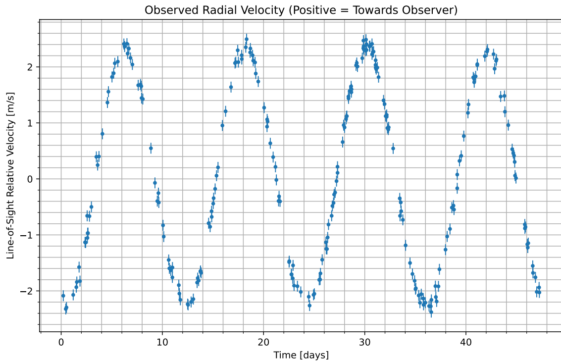
Figure 1: We have isolated the radial velocity of the host star due to the candidate planet. Data begins at UTC 2091-01-15/09:30. Positive values indicate the velocity at which the star is moving towards us; negative indicate the velocity at which it is moving away.
