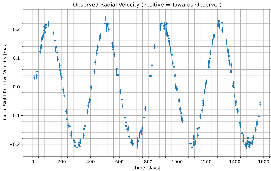
Figure 1: We have isolated the radial velocity of the host star due to the candidate planet. Data begins at UTC 2081-01-28/11:18. Positive values indicate the velocity at which the star is moving towards us; negative indicate the velocity at which it is moving away.
