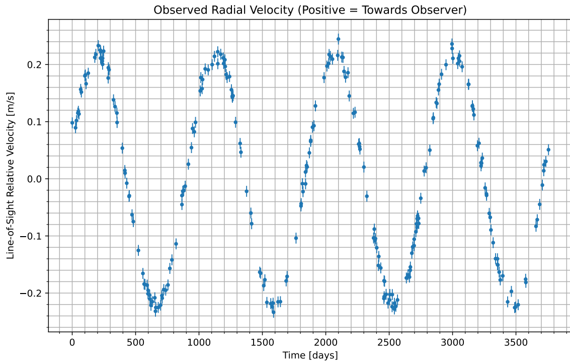
Figure 1: We have isolated the radial velocity of the host star due to the candidate planet. Data begins at UTC 2060-08-29/16:00. Positive values indicate the velocity at which the star is moving towards us; negative indicate the velocity at which it is moving away.
