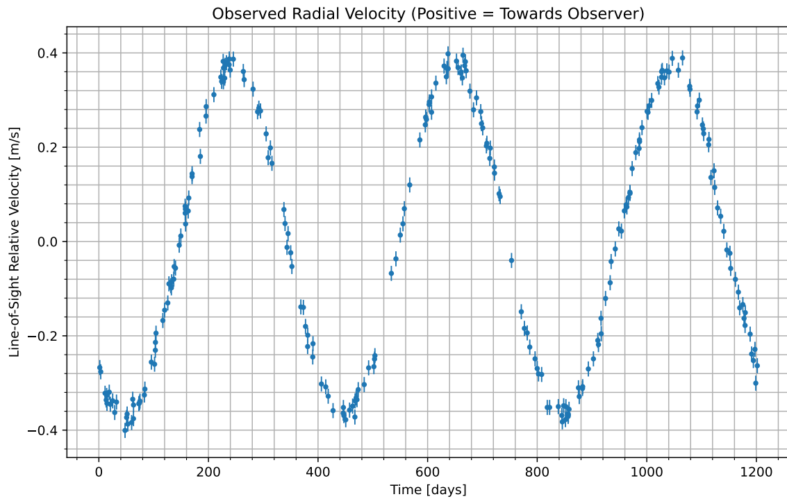
Figure 1: We have isolated the radial velocity of the host star due to the candidate planet. Data begins at UTC 2079-01-05/09:31. Positive values indicate the velocity at which the star is moving towards us; negative indicate the velocity at which it is moving away.
