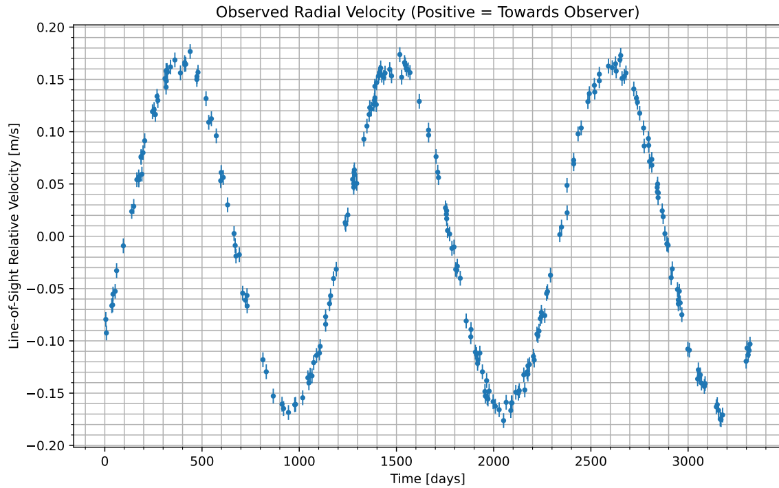
Figure 1: We have isolated the radial velocity of the host star due to the candidate planet. Data begins at UTC 2077-06-15/00:33. Positive values indicate the velocity at which the star is moving towards us; negative indicate the velocity at which it is moving away.
