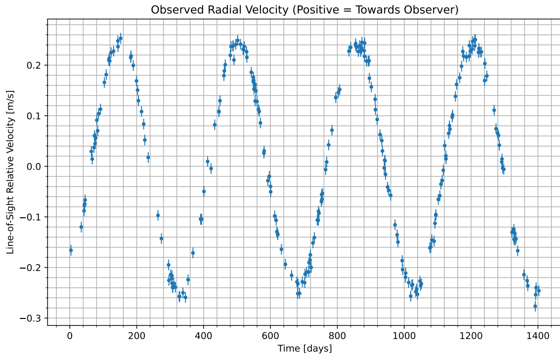
Figure 1: We have isolated the radial velocity of the host star due to the candidate planet. Data begins at UTC 2072-03-15/15:49. Positive values indicate the velocity at which the star is moving towards us; negative indicate the velocity at which it is moving away.
