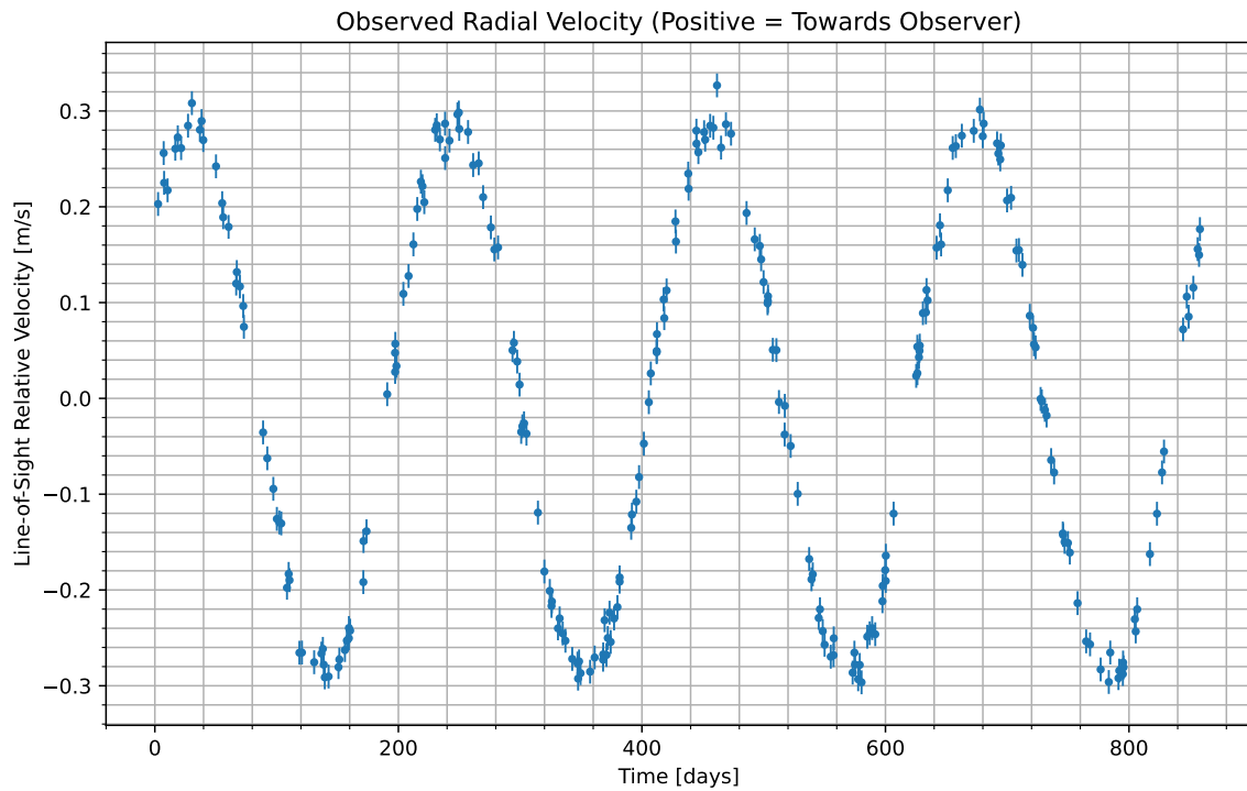
Figure 1: We have isolated the radial velocity of the host star due to the candidate planet. Data begins at UTC 2081-04-17/02:09. Positive values indicate the velocity at which the star is moving towards us; negative indicate the velocity at which it is moving away.
