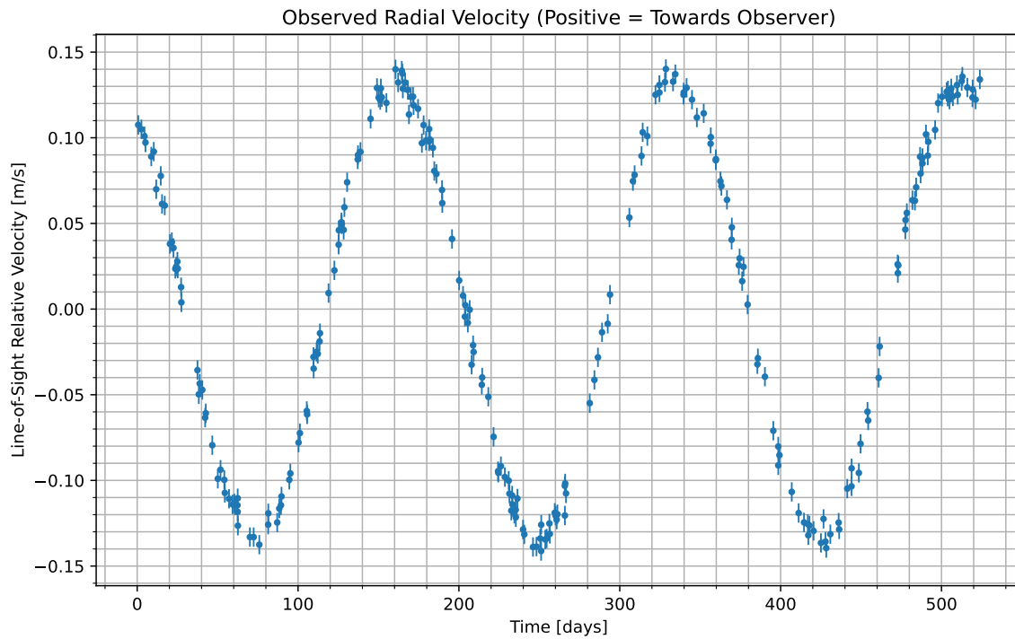
Figure 1: We have isolated the radial velocity of the host star due to the candidate planet. Data begins at UTC 2084-08-17/20:00. Positive values indicate the velocity at which the star is moving towards us; negative indicate the velocity at which it is moving away.
