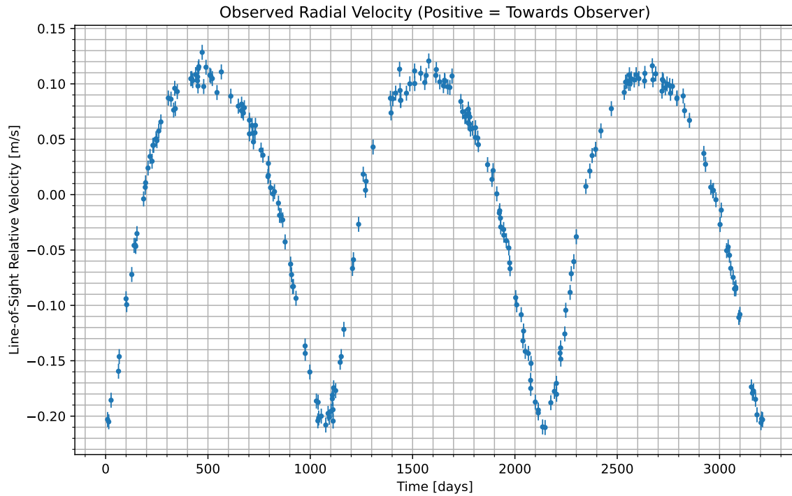
Figure 1: We have isolated the radial velocity of the host star due to the candidate planet. Data begins at UTC 2082-08-24/20:20. Positive values indicate the velocity at which the star is moving towards us; negative indicate the velocity at which it is moving away.
