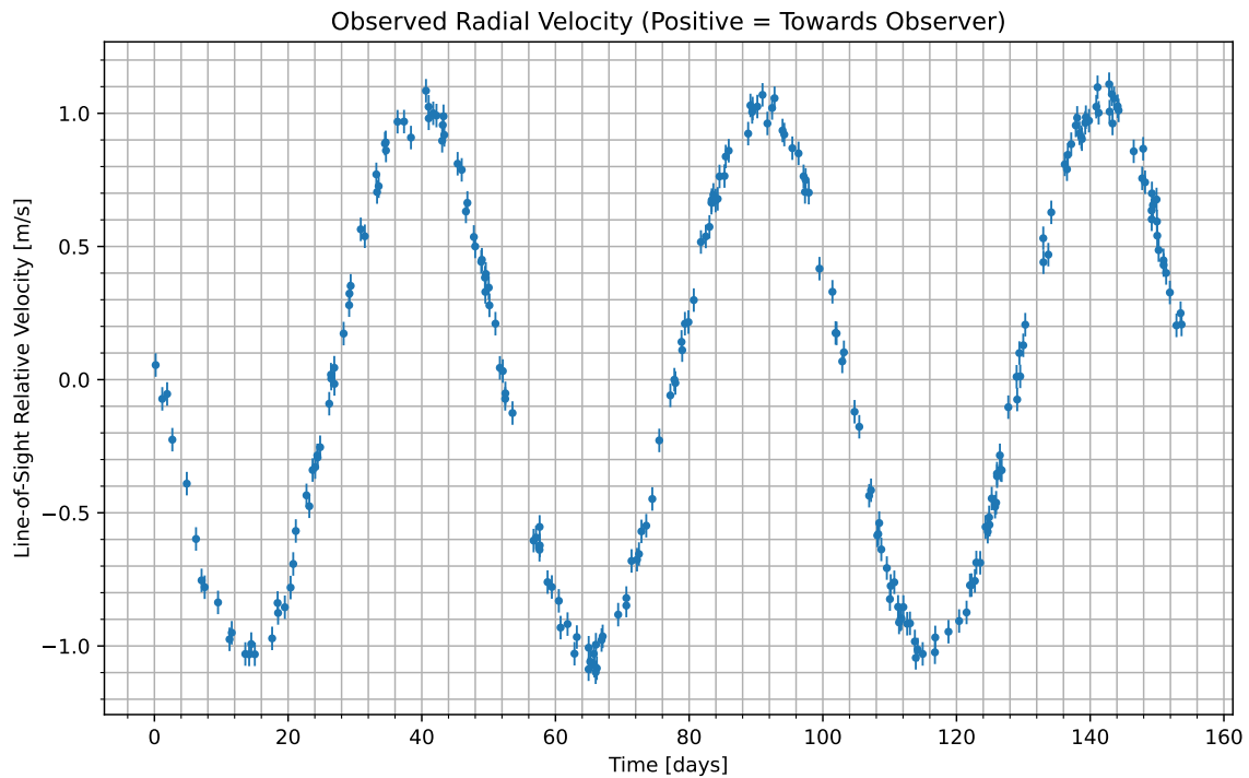
Figure 1: We have isolated the radial velocity of the host star due to the candidate planet. Data begins at UTC 2071-06-24/22:47. Positive values indicate the velocity at which the star is moving towards us; negative indicate the velocity at which it is moving away.
