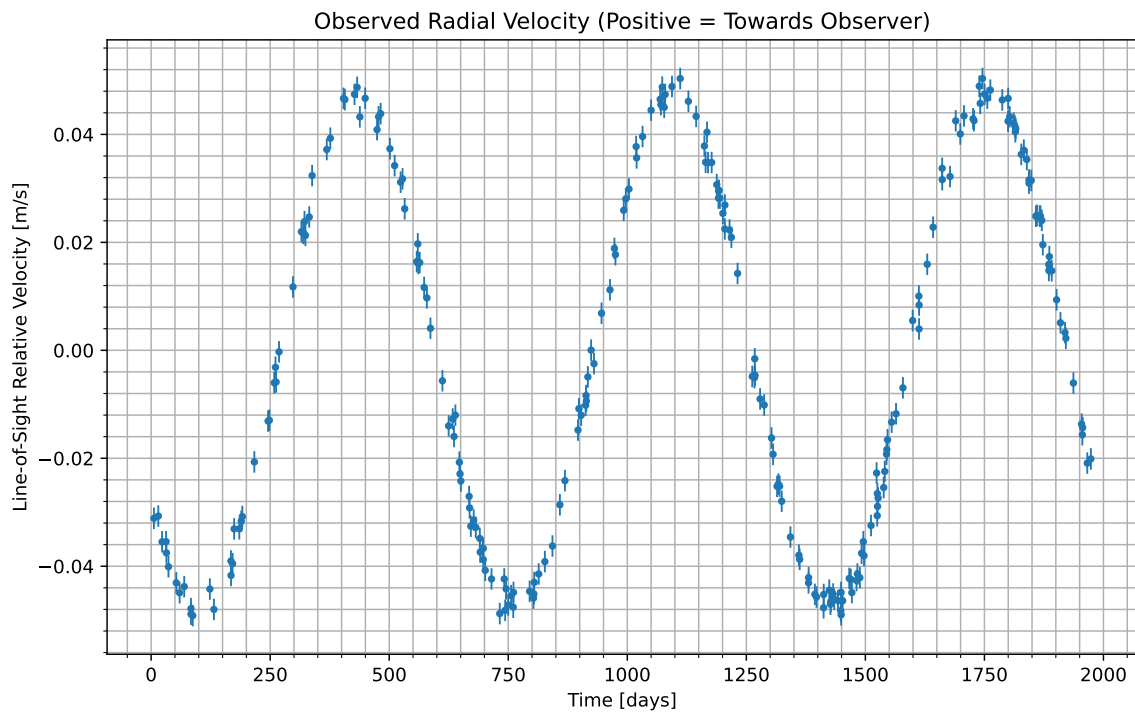
Figure 1: We have isolated the radial velocity of the host star due to the candidate planet. Data begins at UTC 2080-12-26/04:18. Positive values indicate the velocity at which the star is moving towards us; negative indicate the velocity at which it is moving away.
