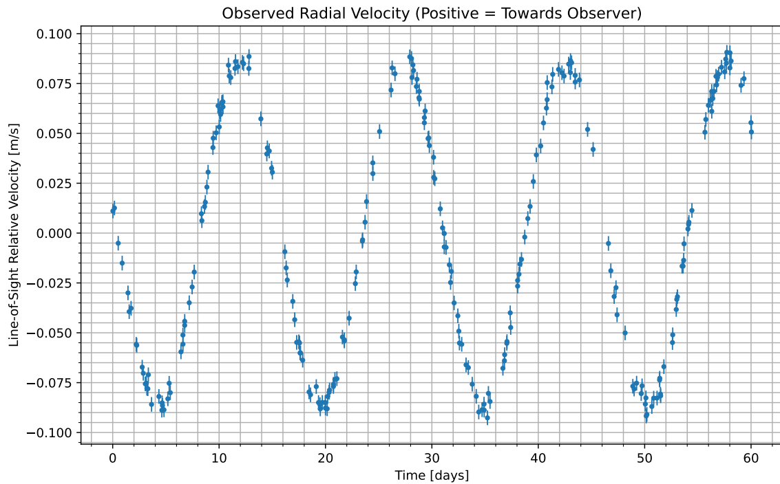
Figure 1: We have isolated the radial velocity of the host star due to the candidate planet. Data begins at UTC 2074-01-14/07:28. Positive values indicate the velocity at which the star is moving towards us; negative indicate the velocity at which it is moving away.
