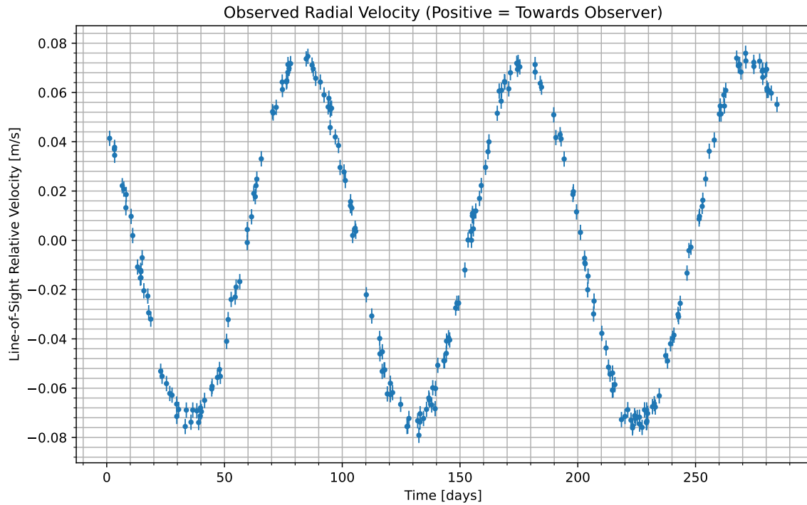
Figure 1: We have isolated the radial velocity of the host star due to the candidate planet. Data begins at UTC 2086-11-06/20:07. Positive values indicate the velocity at which the star is moving towards us; negative indicate the velocity at which it is moving away.
