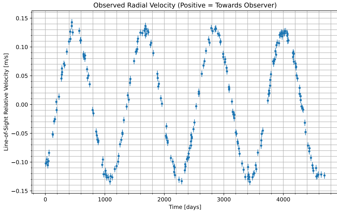
Figure 1: We have isolated the radial velocity of the host star due to the candidate planet. Data begins at UTC 2062-11-12/19:18. Positive values indicate the velocity at which the star is moving towards us; negative indicate the velocity at which it is moving away.
