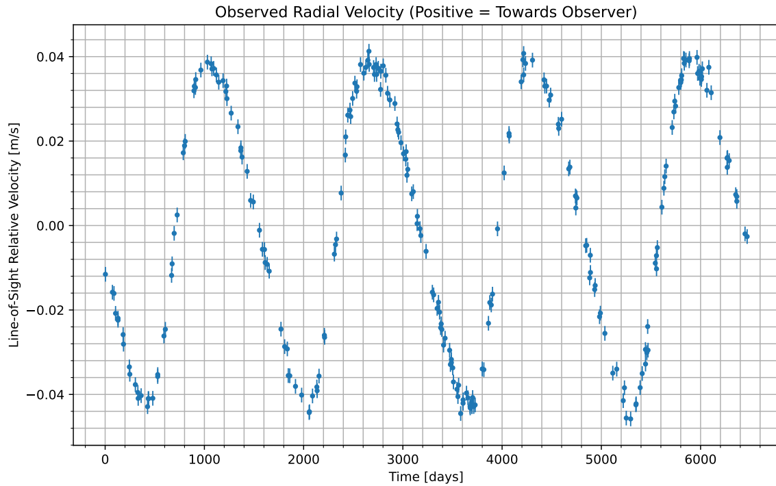
Figure 1: We have isolated the radial velocity of the host star due to the candidate planet. Data begins at UTC 2059-01-27/01:39. Positive values indicate the velocity at which the star is moving towards us; negative indicate the velocity at which it is moving away.
